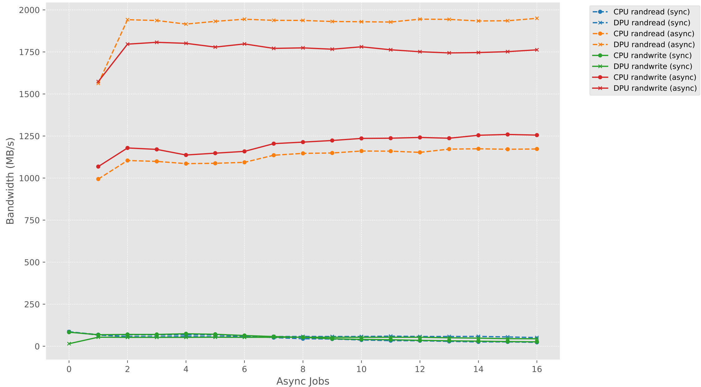
Bandwidth vs Async Jobs (sync1_asyncN) - RAND (CPU vs DPU)
